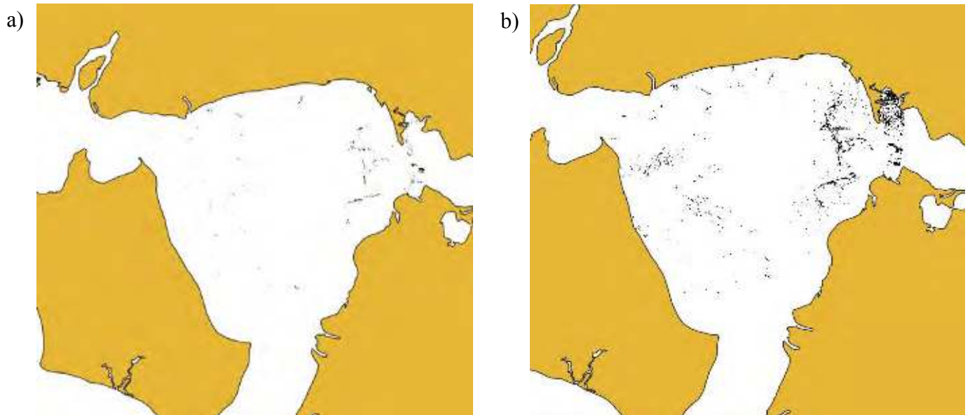
b) Math band: fai > -0.004 and L2 flags = 0
