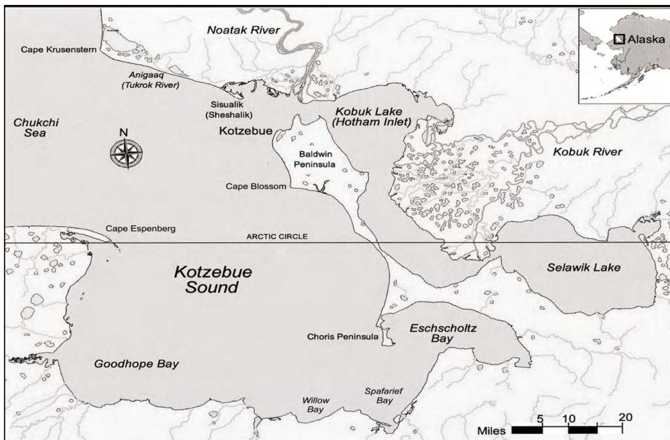
Figure 1: The map of Kotzebue Sound and surrounding areas. (Whiting et al, 2011)
