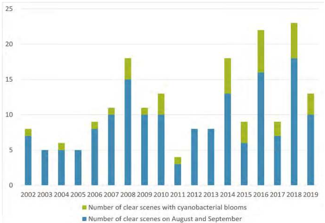
Figure 3: The bar chart shows the amount of clear scenes and the number of scenes with cyanobacterial blooms detected during August and September when the blooms are most likely to be detected.
