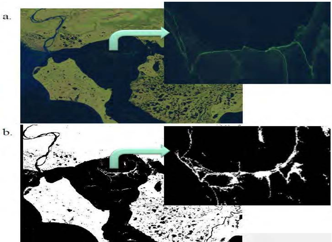
Figure 2a. A true color image downloaded from Sentinel- 2 showing an extensive cyanobacterial blooms on August 29, 2016.
